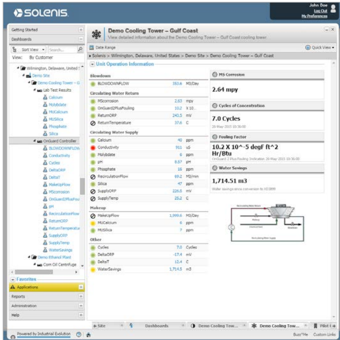
Unit operation dashboard
