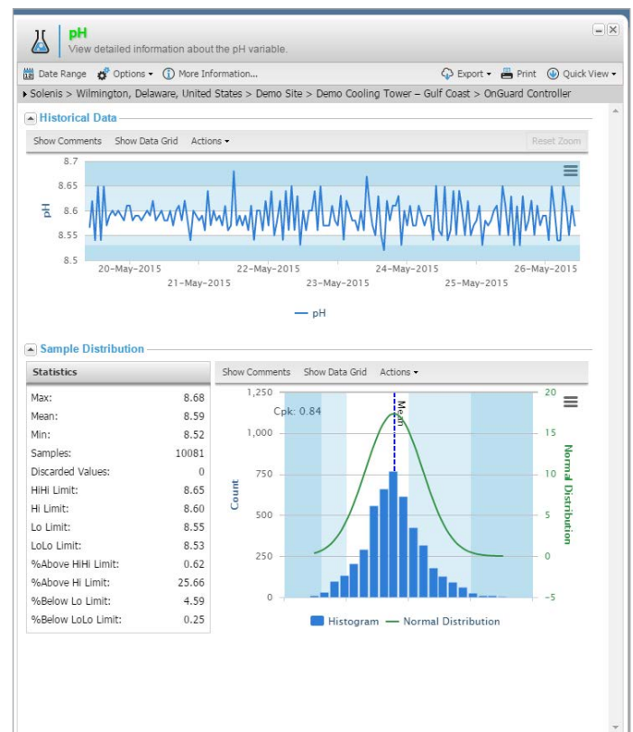
Statistical Process Control graphs
